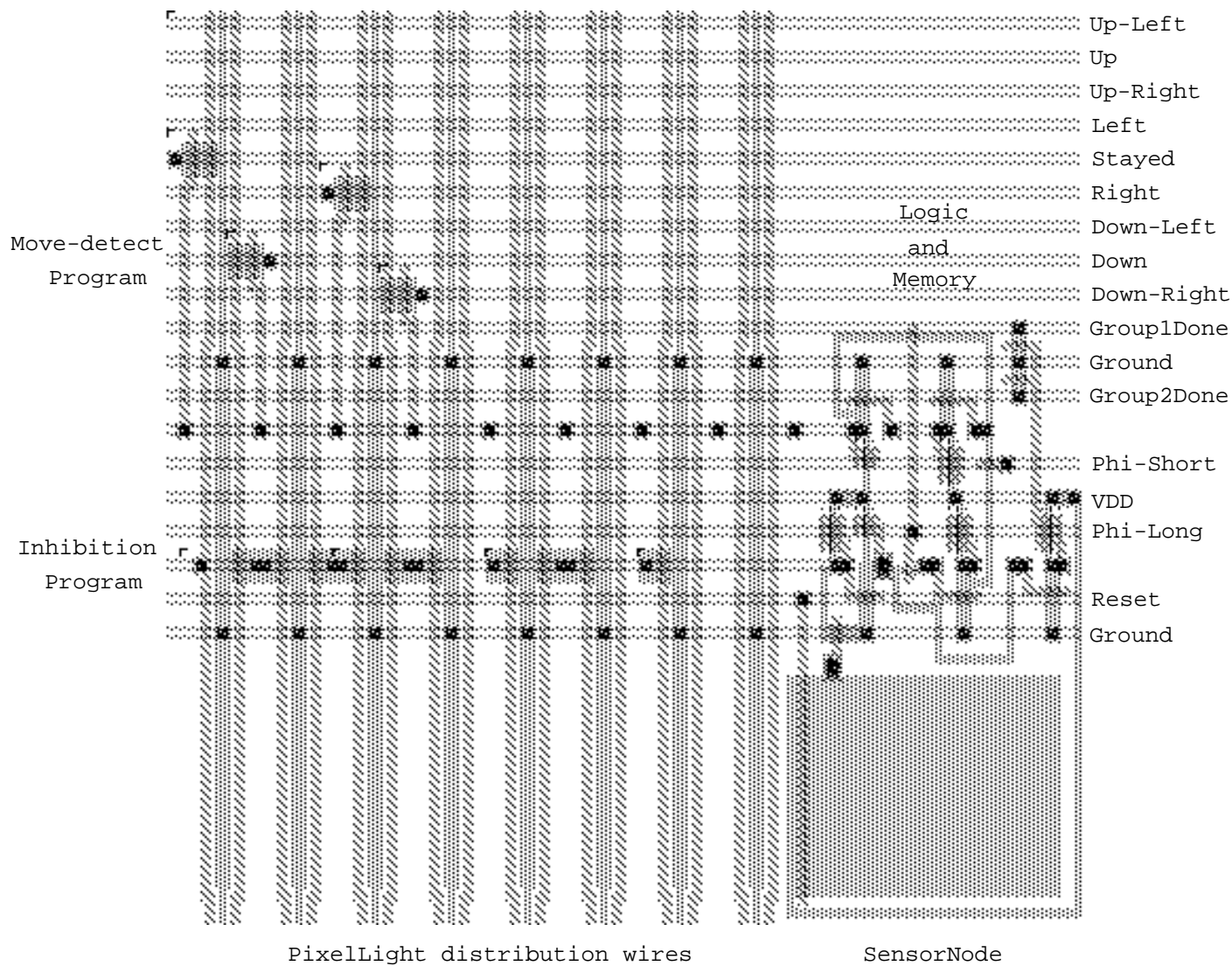
Figure 13. The layout of the upper-left Optical Mouse Cell
