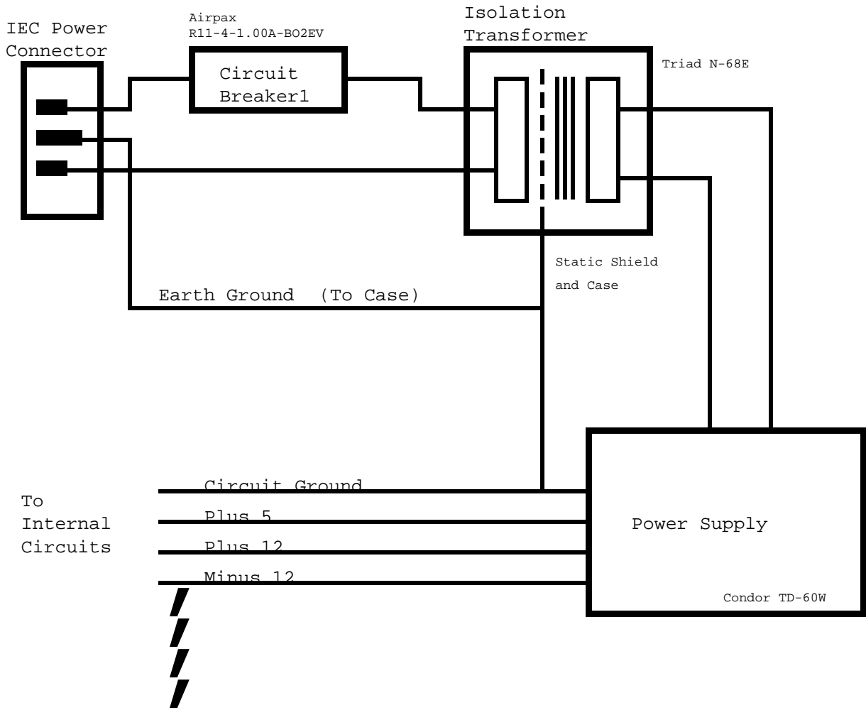
CSL-8308 Power Supply Primary Wiring
