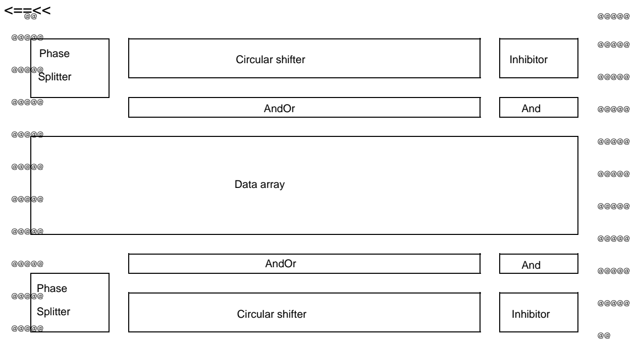
Fig. 3. Structure of FIFO queue
