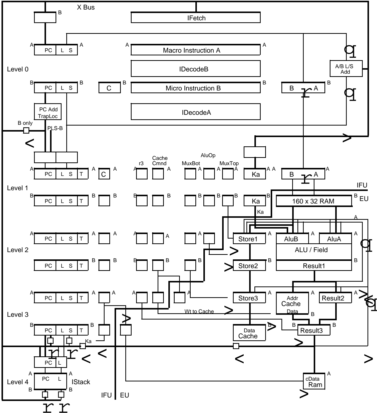
Dragon Processor Pipeline Figure 2
