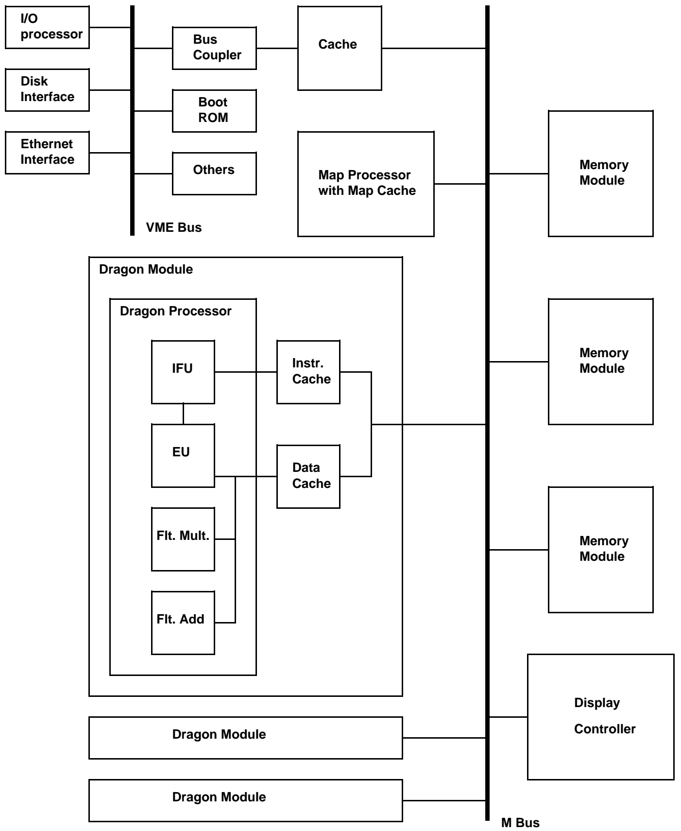
Figure 1. A Dragon Cluster
