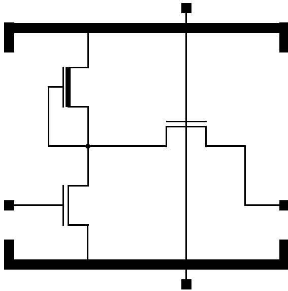
Fig. 7. Basic Shift Register Circuit
