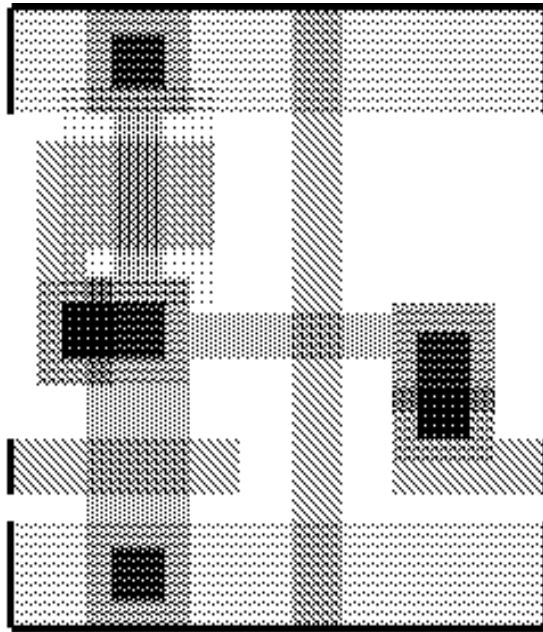
Fig. 6. Basic Shift Register Cell
