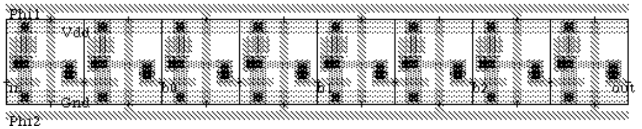
Fig. 5. A Four Bit Shift Register
