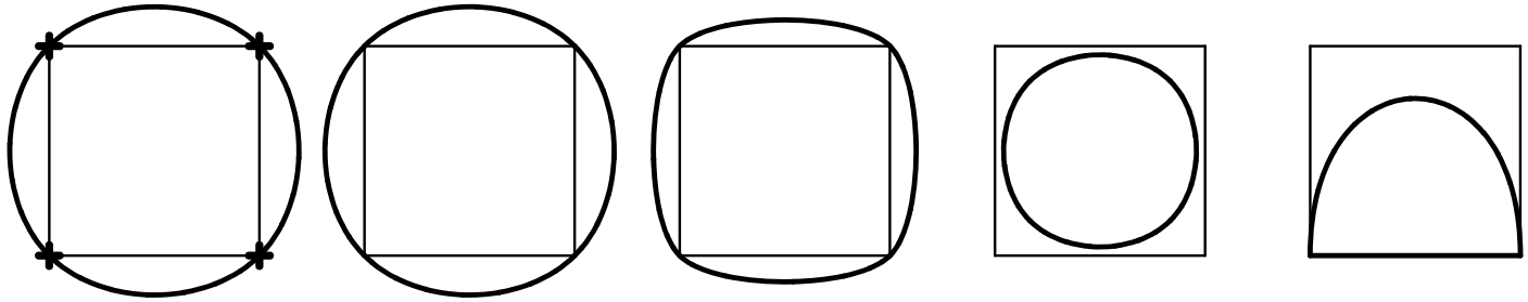
Natural Arc Length
