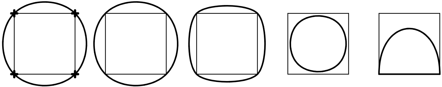
Natural Arc Length
