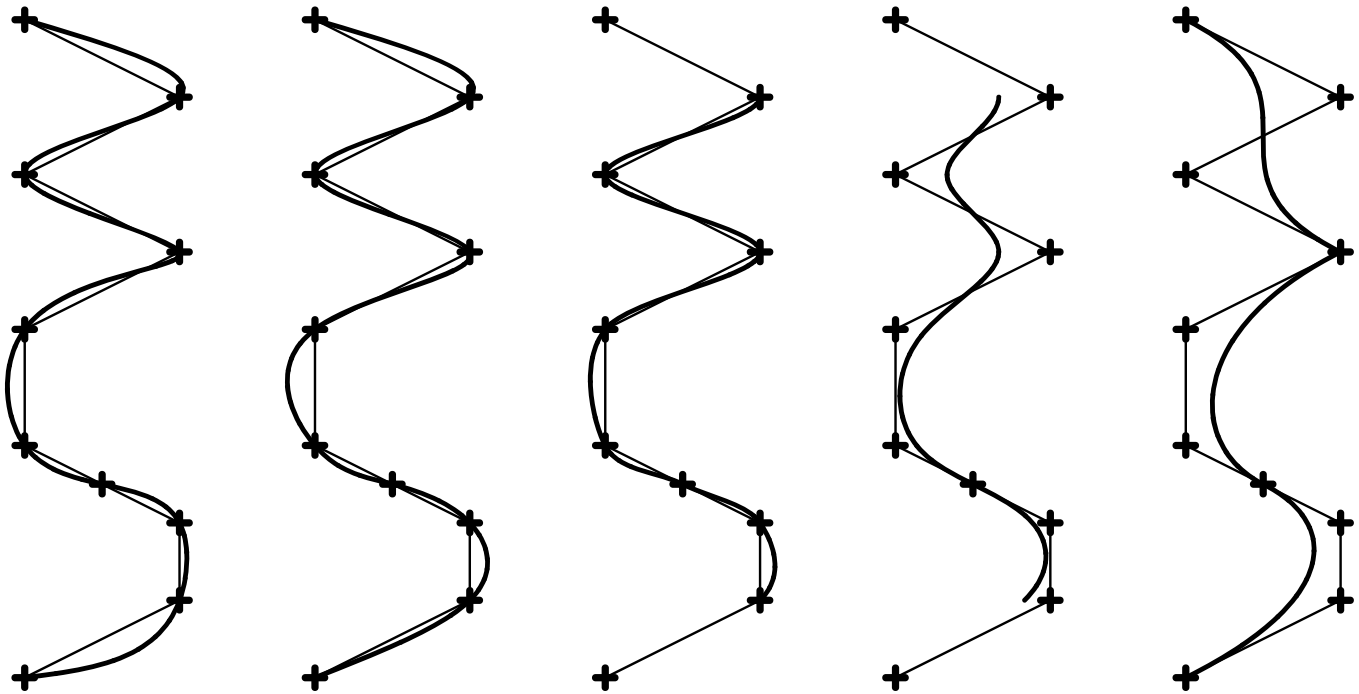
Natural Arc Length
