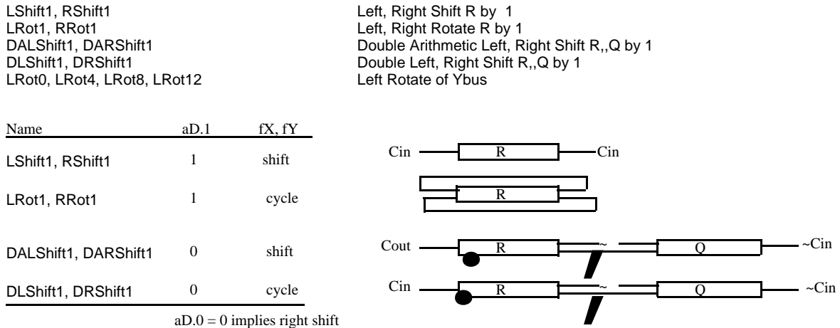
Figure 3. Single Bit Shifting & Rotating
